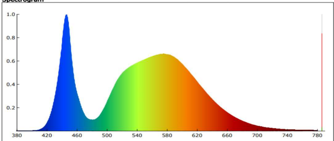
Spectrogram
