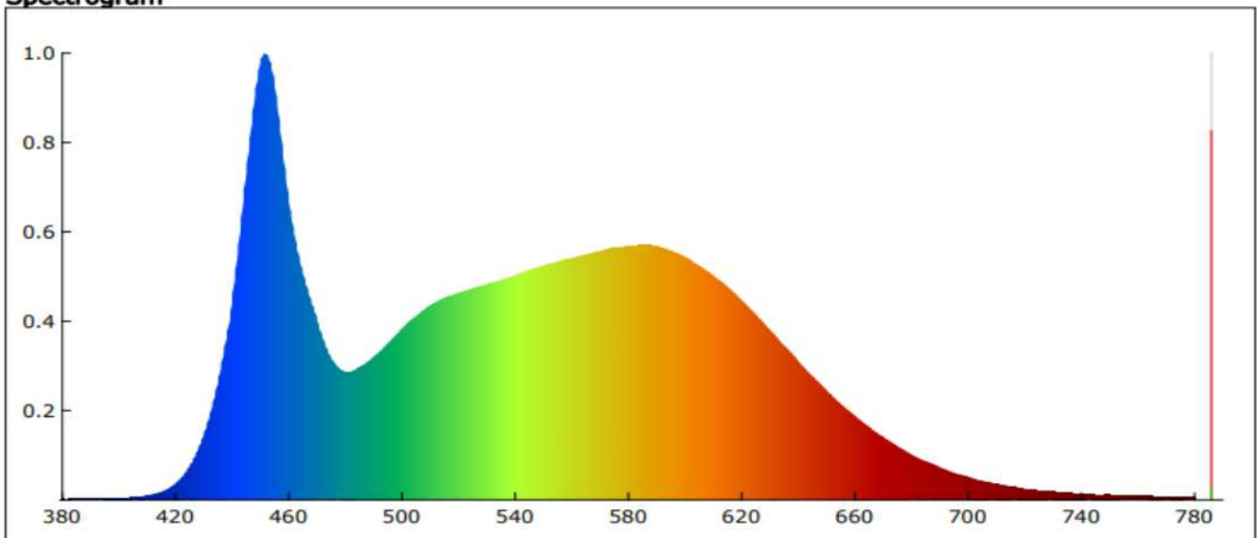
Spectrogram
